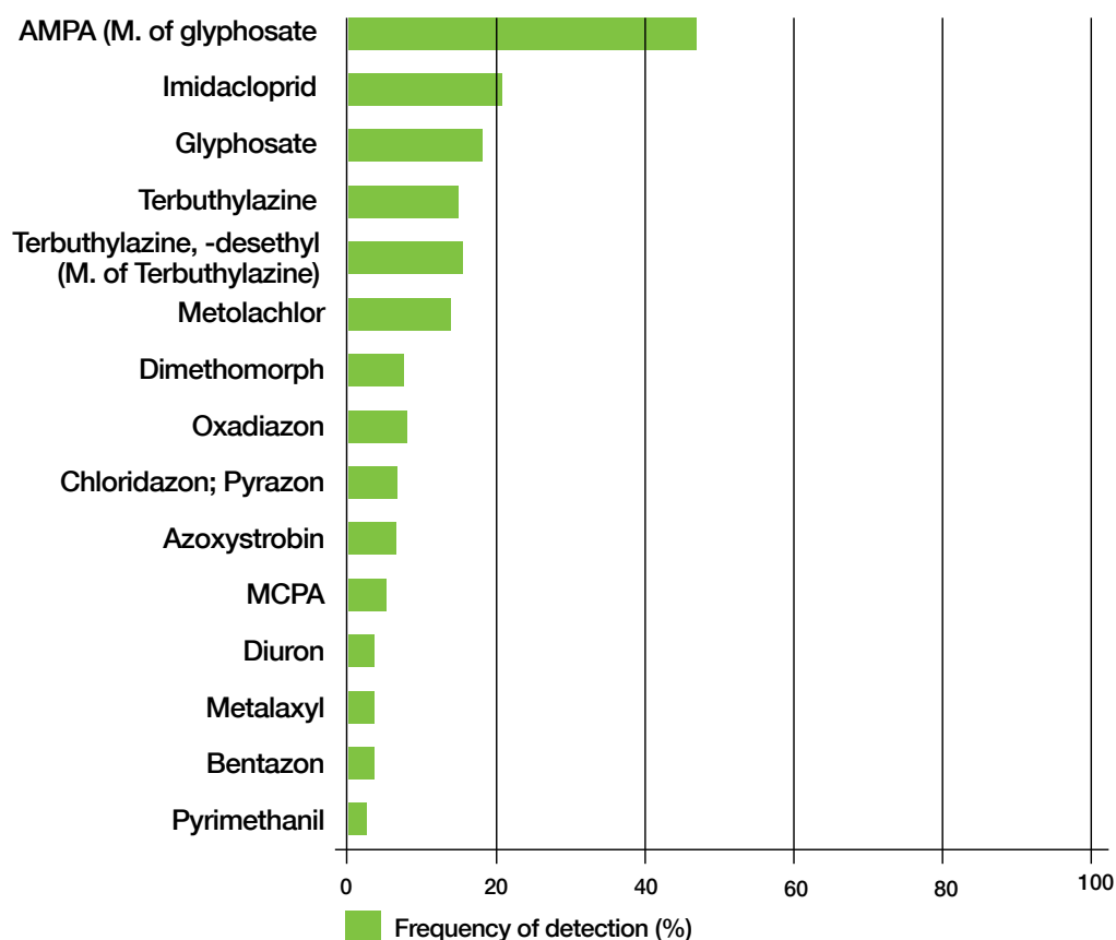
Fig 13: Frequency of detection in surface waters in Italy 2012 (ISPRA 2014)
