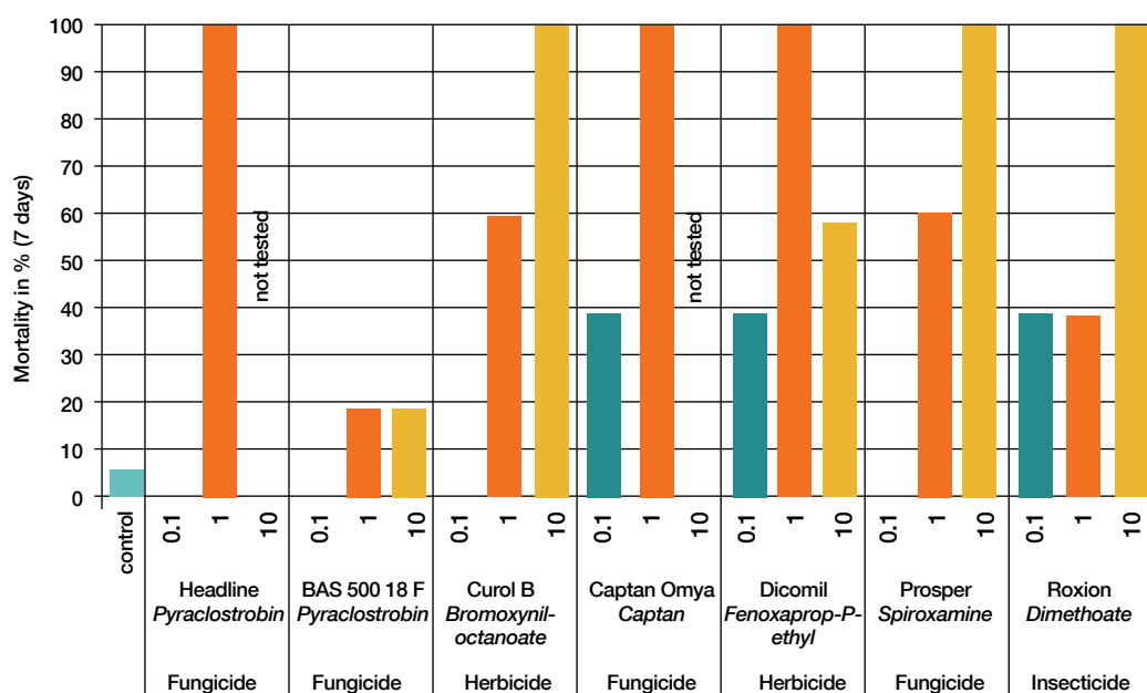
Fig 6: Frog Mortality
