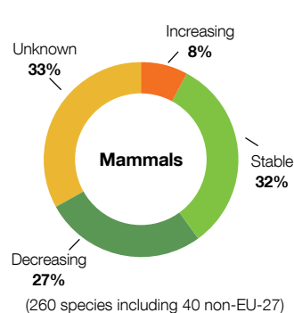
Figure 3: Population Trends
